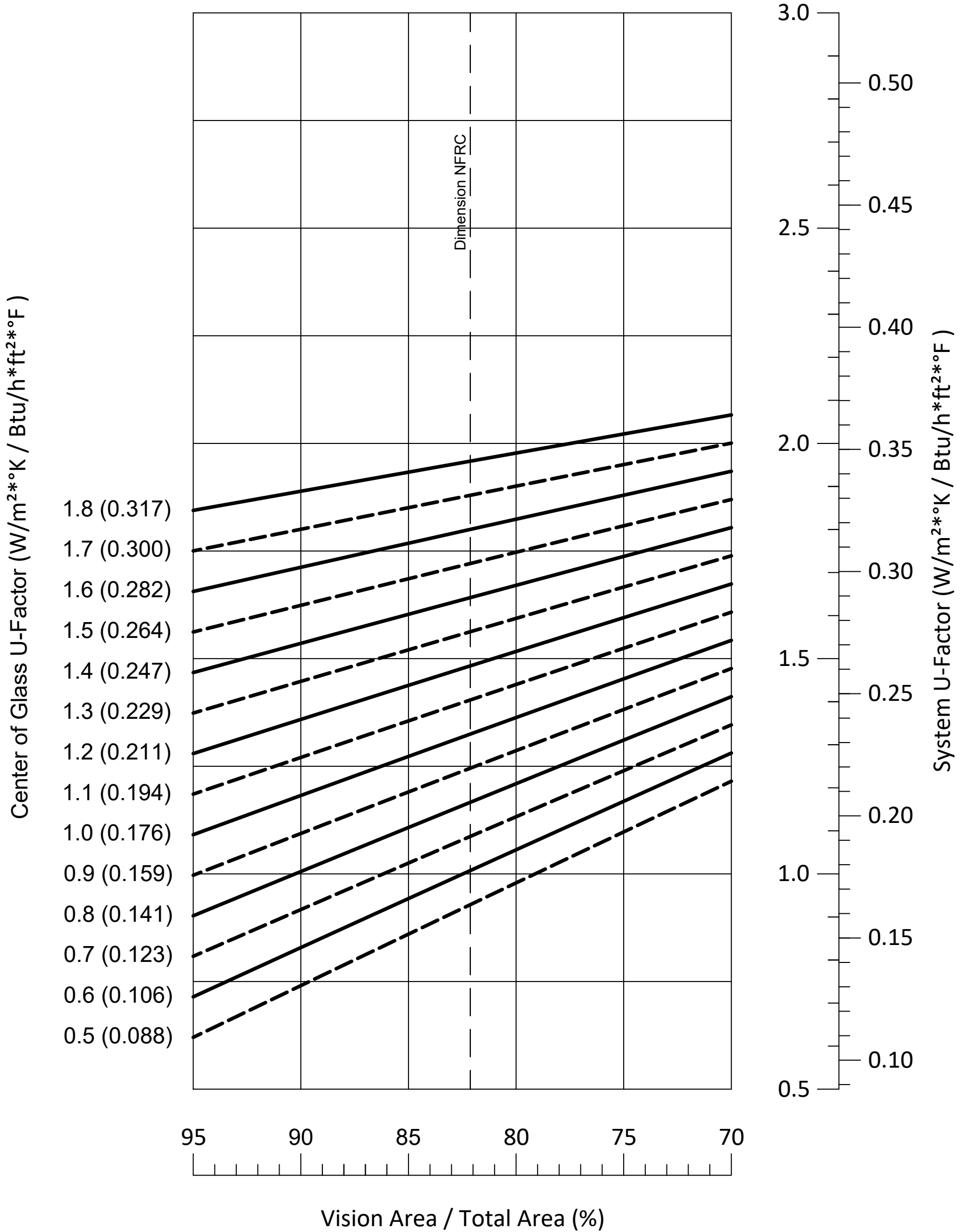
System U-Factor vs. Percentage of Vision Area
